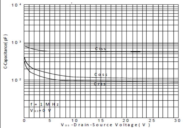
Figure 8. Typical Capacitance vs. Drain-to-Source Voltage
